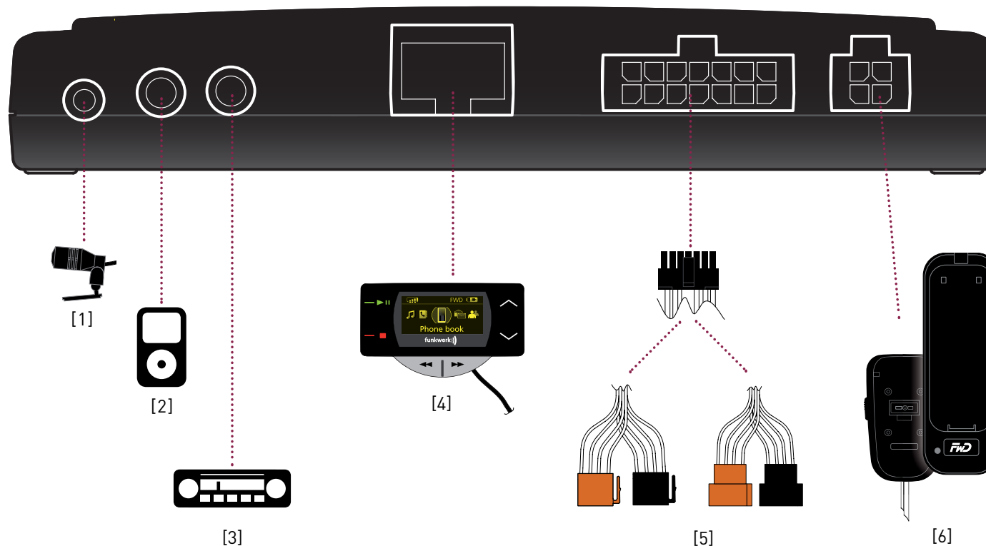
Fig. 13: Electronics box connection
