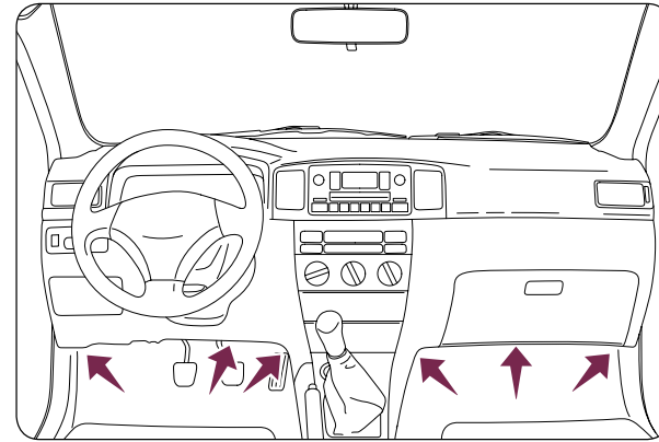
Fig. 03: Installation locations for the elec- tronics box
