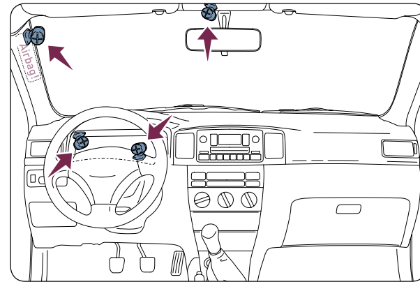
Fig. 04: Installation location for microphone
