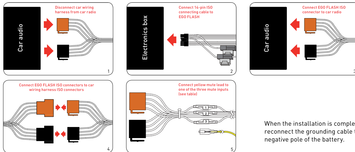
Fig. 07: Installation procedure
